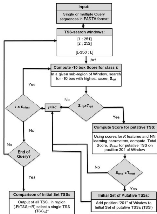
Fig. 1. Flow-chart of the algorithm implemented in the bTSSfinder program. T_{i,10} is the threshold for the prediction of the -10 box (specific for every sigma class). T_{total} – the NN threshold for the selection of TSSs
