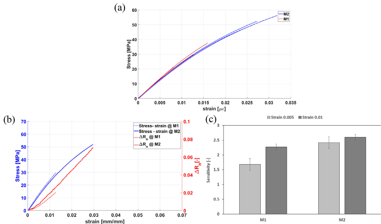
Figure 7. (a) stress-strain curve for three samples tested, piezoresistivity behavior of the nanocomposites during tensile test, (c) sensitivity.
