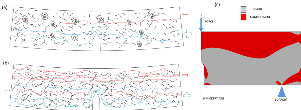
Figure 9. (a-b) Schematic illustration of formation and breakage of electrical pathways during fracture test in M1 and M2 batches respectively, (c) tension and compression stress distributions in the SENB specimen, results based on finite element analysis.
