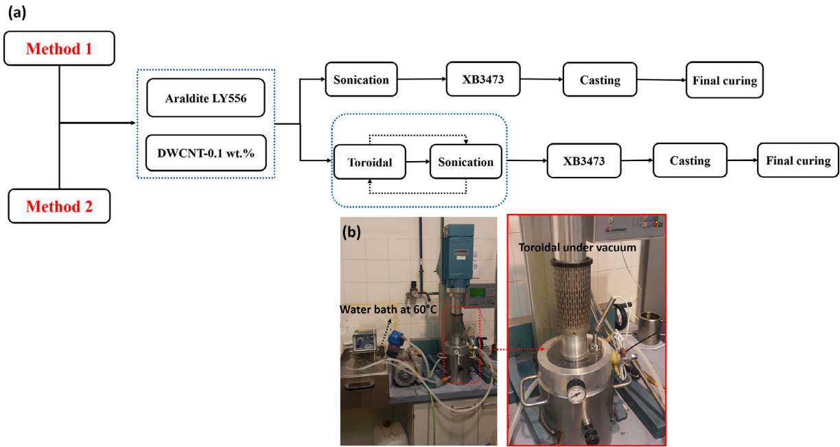
Figure 1. (a) Manufacturing approaches, (b) toroidal stirring with simultaneous degassing at 60 °C.
