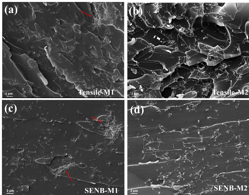
Figure 3. SEM image of the CNT dispersion: (a-b) tensile, (c-d) SENB specimens (left and right figures represent samples produced by M1 and M2 respectively).
