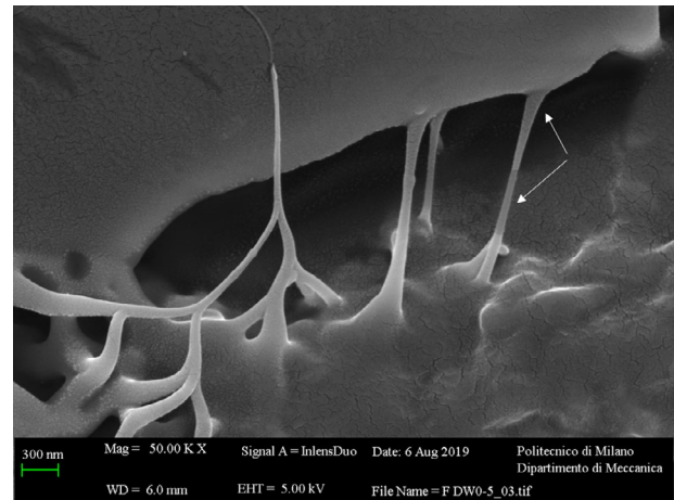
Figure 5. Crack-bridging mechanism of CNTs.
