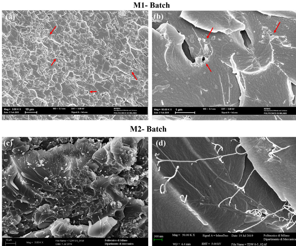
Figure 4. FESEM image of the fracture surface of tensile specimen: (a-b) M1, (c-d) M2, red arrows point to presence of voids.
