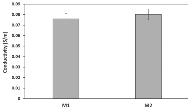
Figure 6. Electrical conductivity for the samples produced by M1 and M2.
