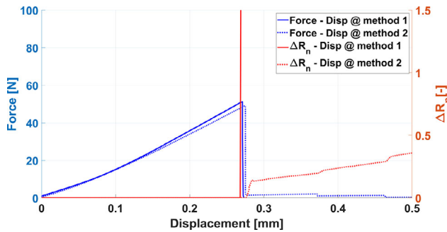
Figure 8. Piezoresistivity behavior during fracture test: (a) before crack extension, (b) after failure.
