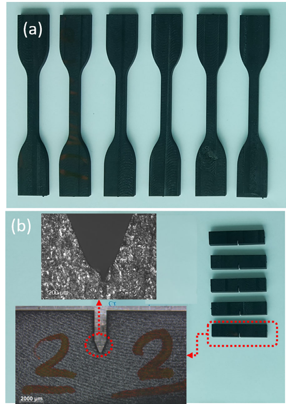
Figure 2. Sample configuration: (a) Dog-bone specimen, (b) SENB specimen.
