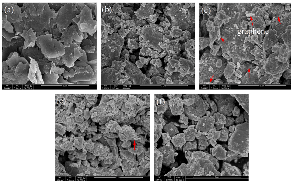
Fig. 5. SEM images for (a) as-received graphene, (b) P-20h, (c) 0.5GNP-10m, (d) 0.05GNP-1m, (e) 0.05GNP-10m and (f) 0.05GNP-20 samples.
