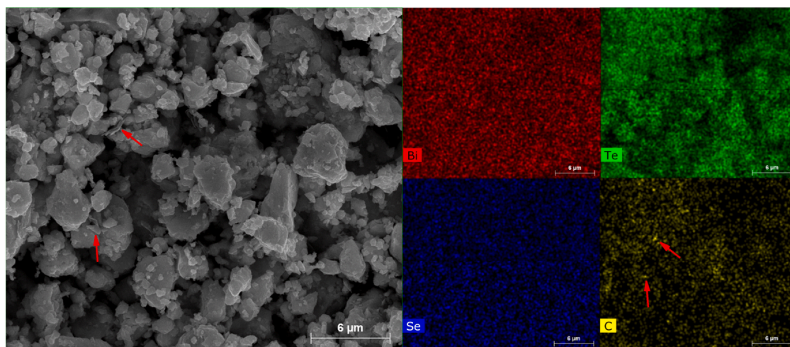
Fig. 6. SEM image with elemental mapping using EDS for milled 0.5GNP-10m sample.
