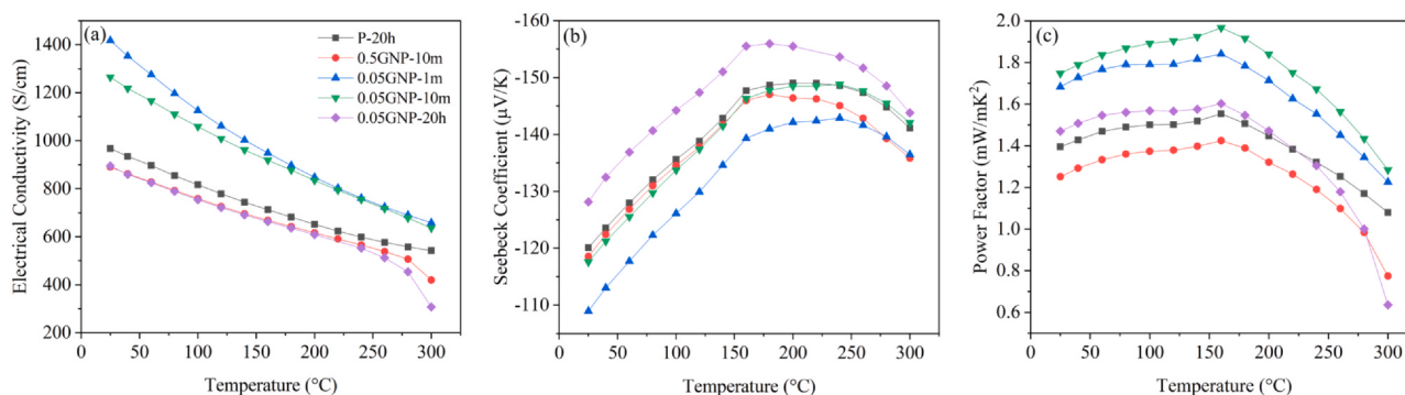
Fig. 9. (a) Electrical conductivity, (b) Seebeck coefficient, and (c) power factor trends for the pristine and GNP-Bi 2 Te 2.7 Se 0.3 composite samples.
